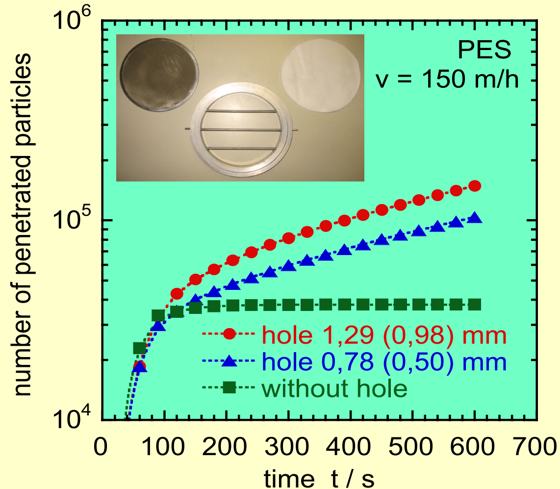
Number of particles on clean gas side with time for different filter media defects
