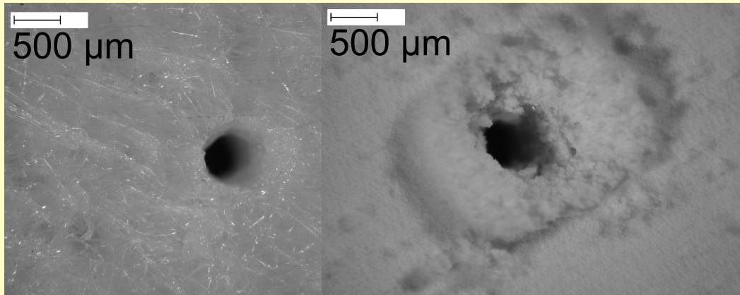
Pinholed polyester needled felt without (left) and with (right) dust particles
